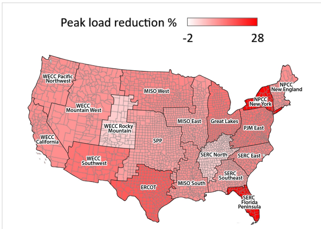
Figure 4-15. Peak electric demand reduction percentage in (top) winter and (bottom) summer at each RAZ resulting from deploying GHPs into 68% of buildings in the United States, coupled with weatherization in single-family homes, in the Grid Decarbonization scenario.
